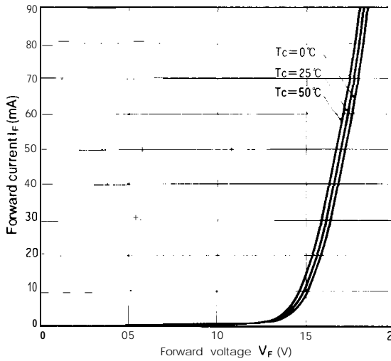
Fig. 00-1 Forward Current vs. Forward Voltage
