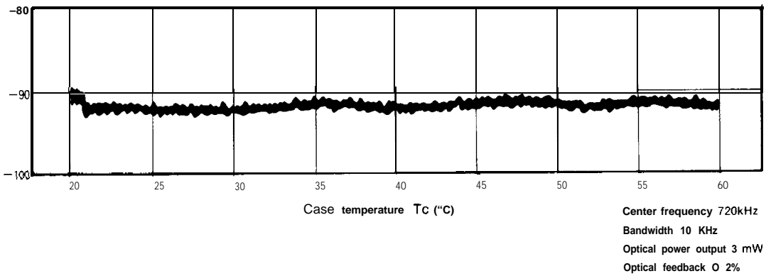
Fig. 61-2 S/N vs. Temperature
