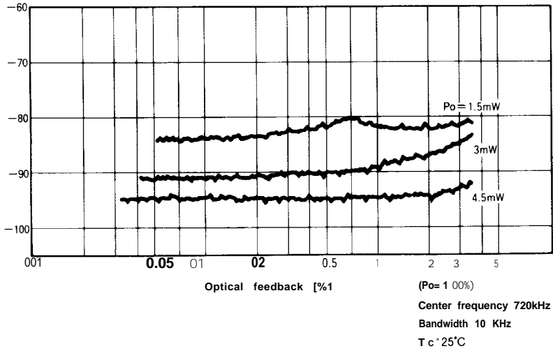
Fig. 61-1 S/N vs. Optical Feedback
